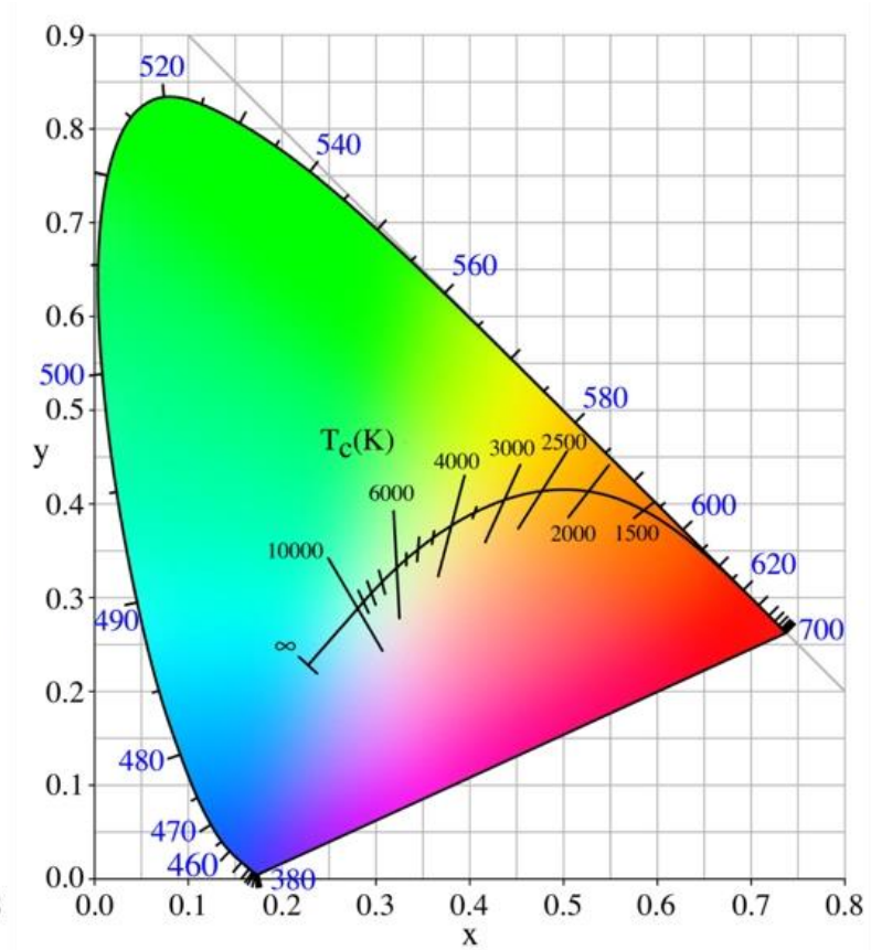
CIEExy1931 - Mapping Colour in Kelvin
