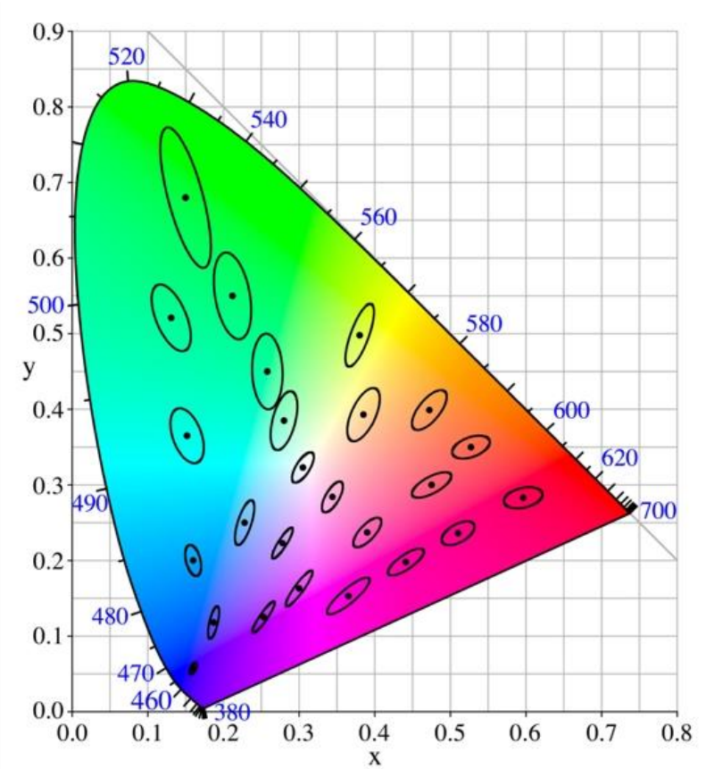
CIEExy1931 - The MacAdams Ellipse
